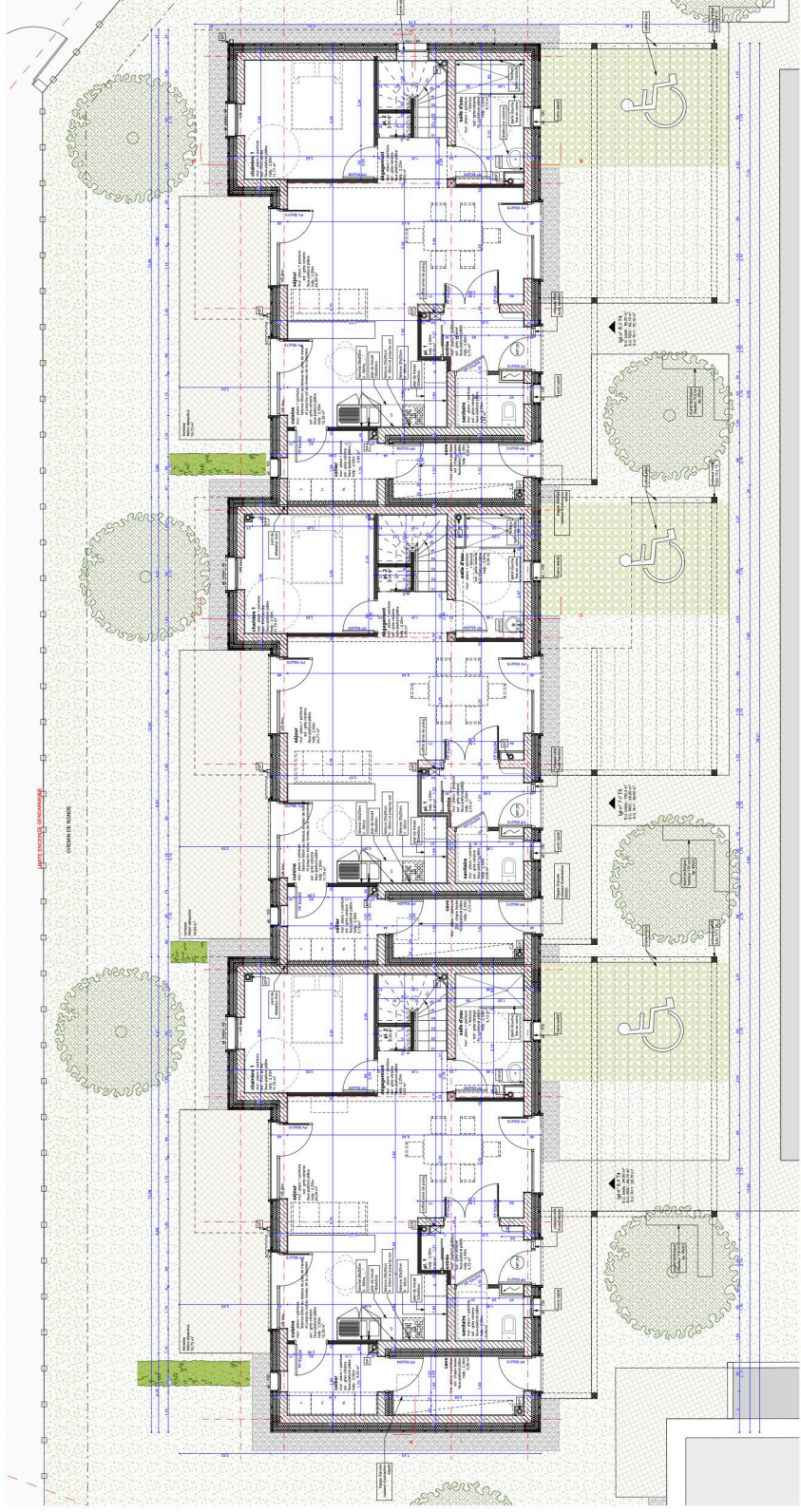
PLAN R+0
